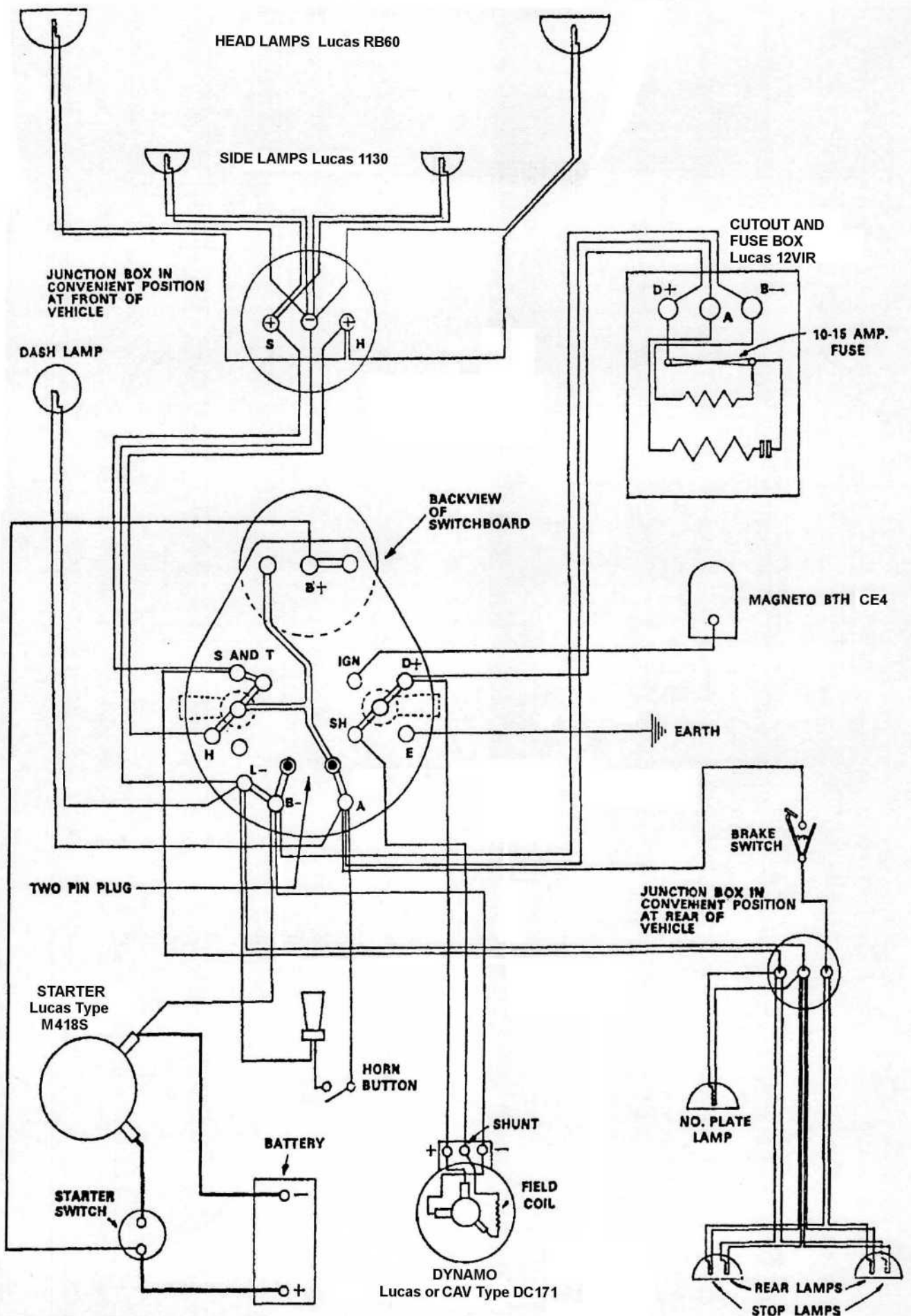
Lucas Wiring Diagram - FWD (based on TA14.75, modified by TC, Aug 2008)
