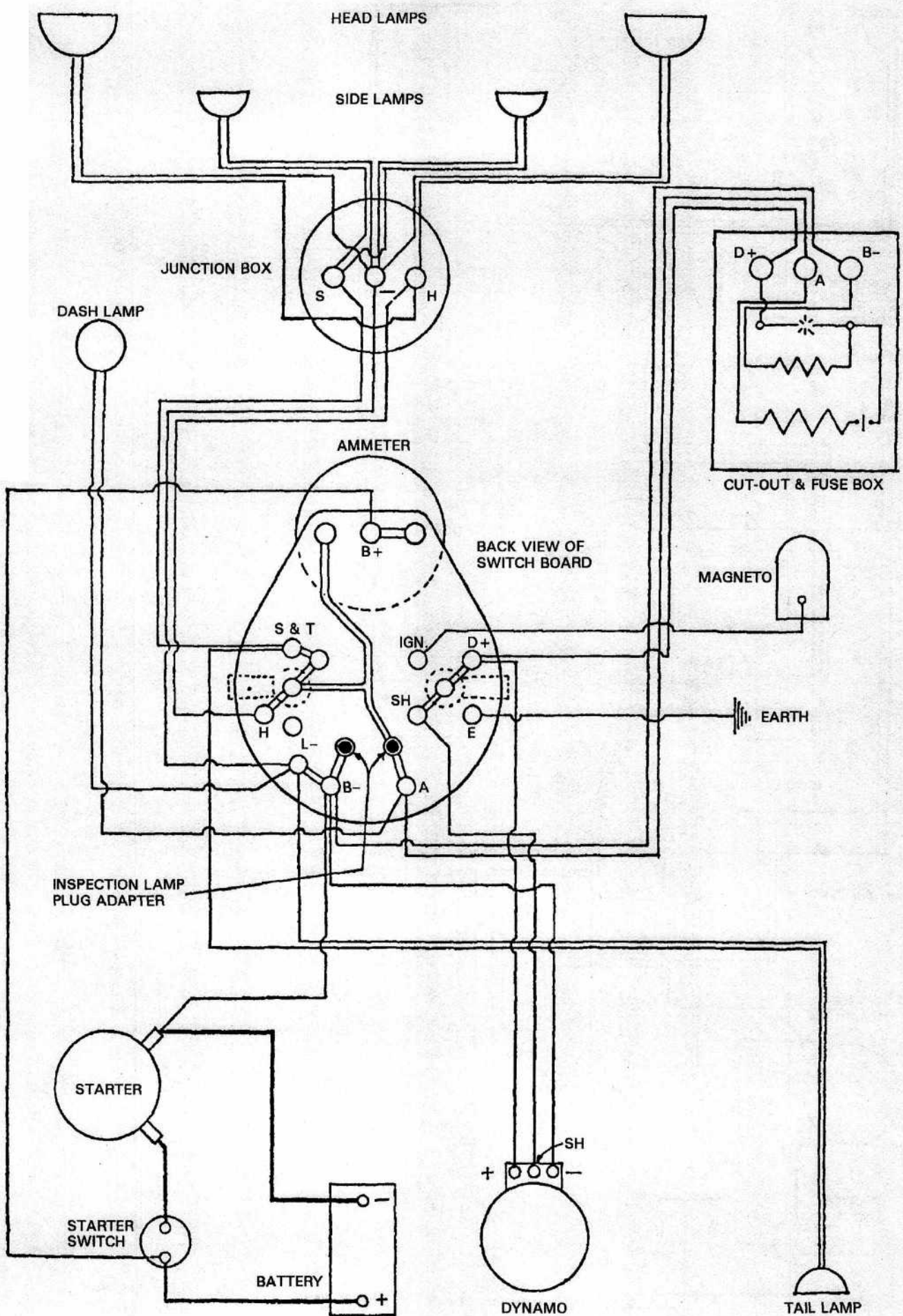
Lucas wiring diagram - 1928 12/50
