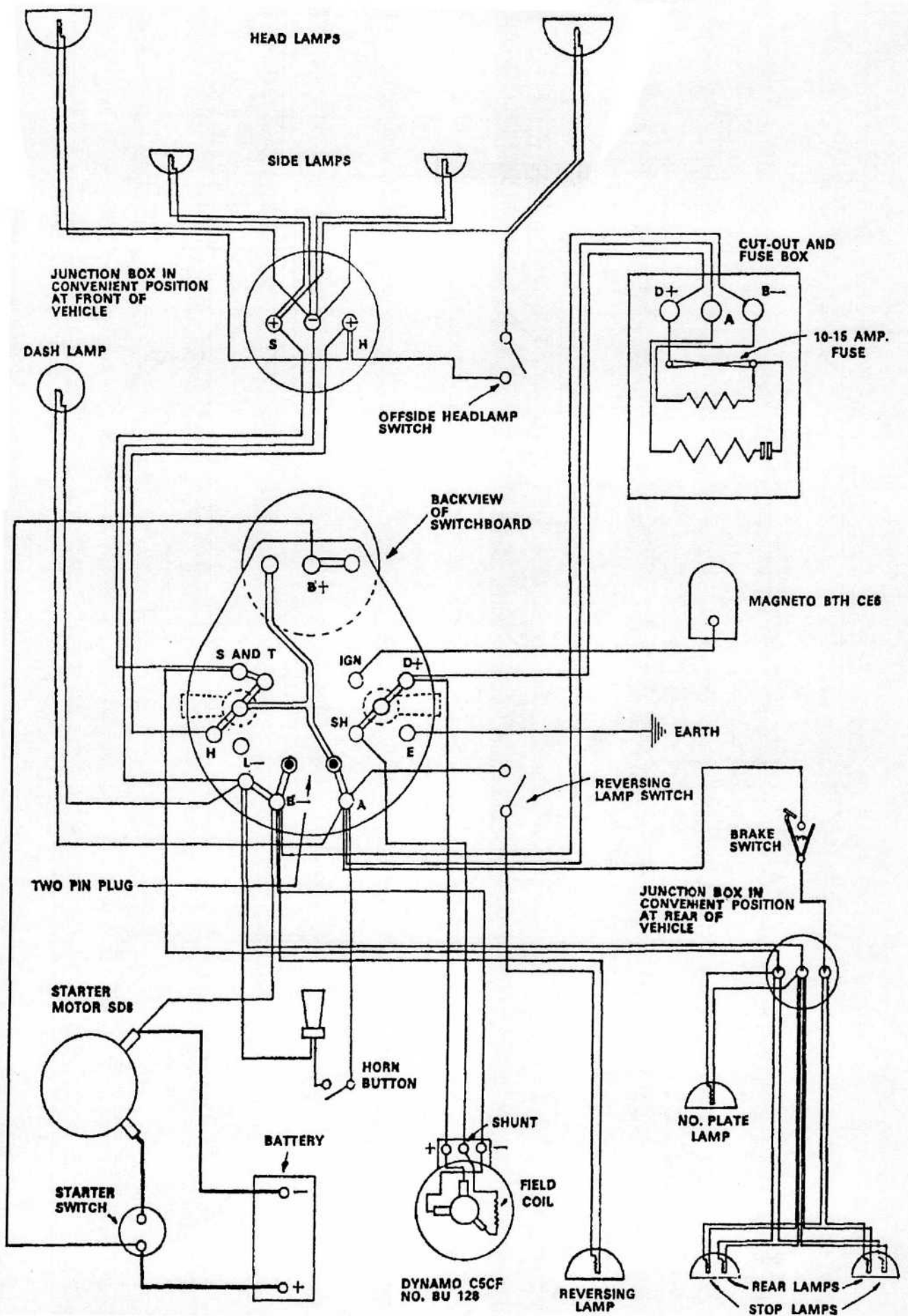
Lucas Wiring Diagram - 1928 TA14.75
